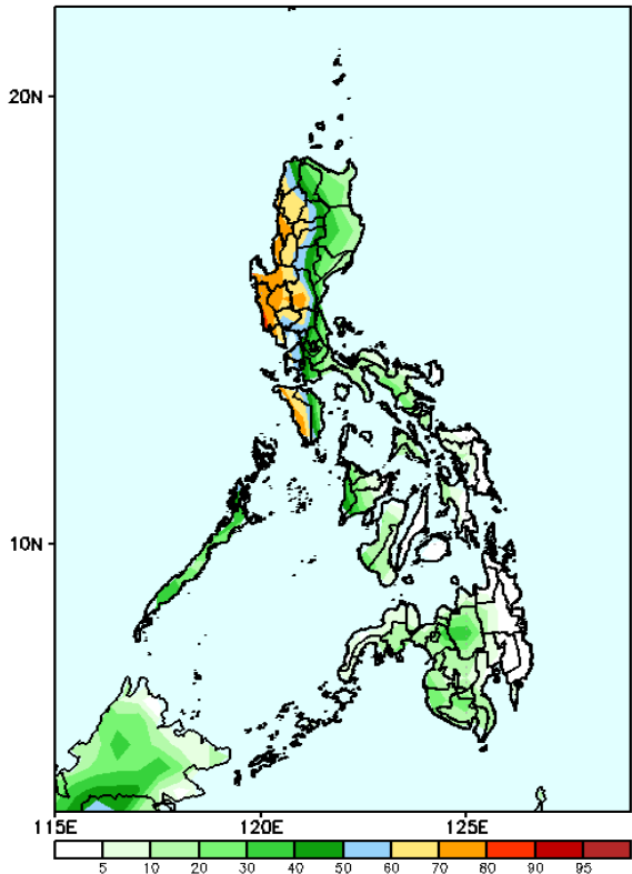
GEFS Week-2 Exceedance Prob. > 100mm Valid: 20230906 – 20230912
