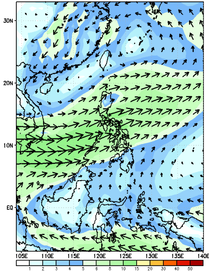
GEFS Week-2 850-hPa Wind Total Valid: 20230906 - 20230912
