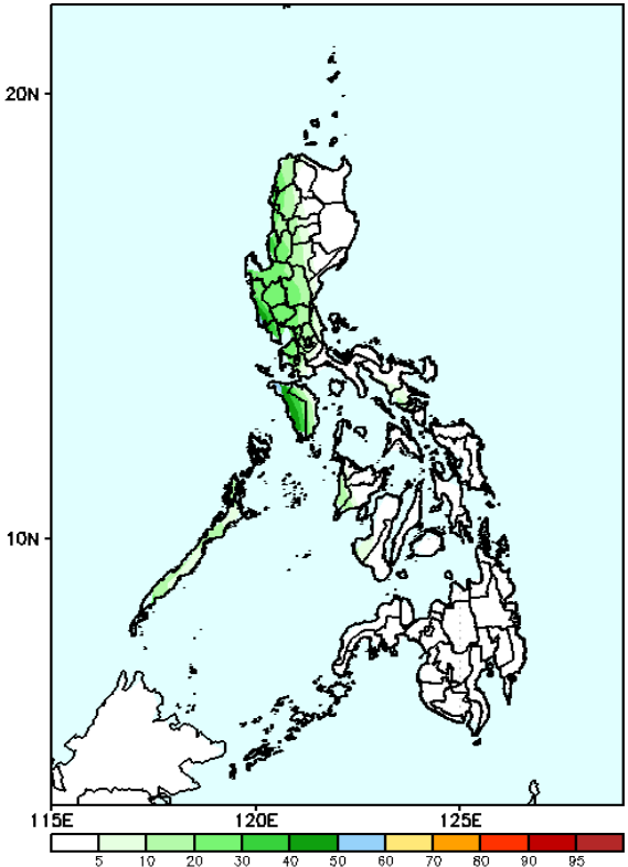
GEFS Week-2 Exceedance Prob. > 200mm Valid: 20230906 – 20230912
