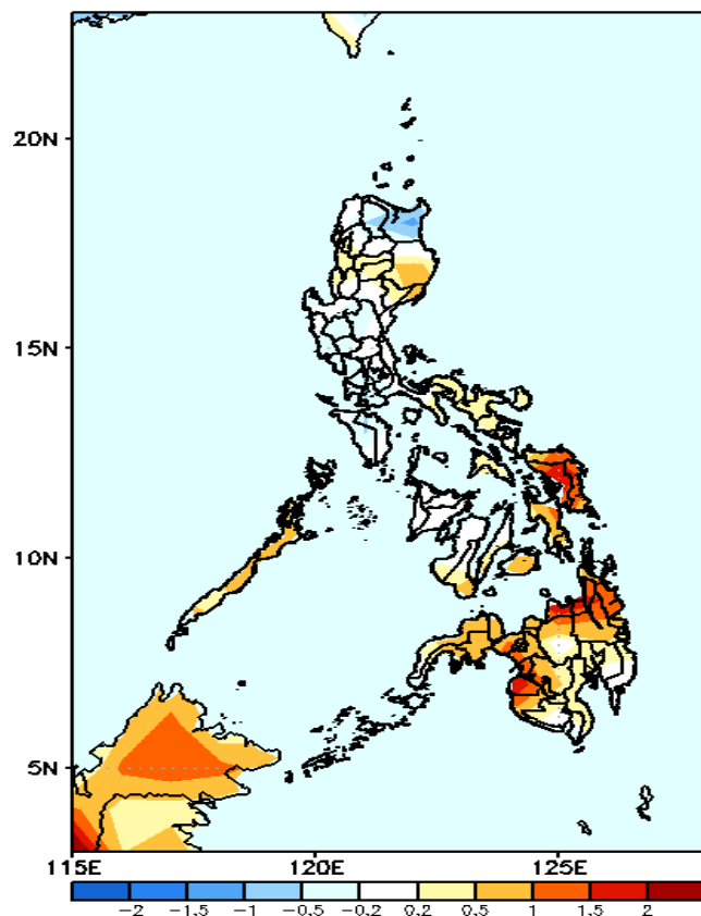
GEFS Week-1 T2m Anomaly Valid: 20230830 - 20230905
