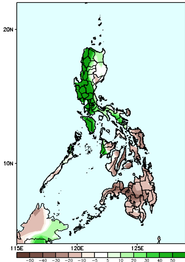
GEFS Week-1 Precip. Anomaly Valid: 20230830 - 20230905
