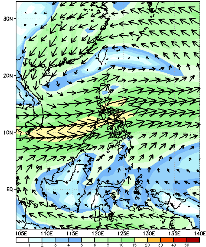
GEFS Week-1 850-hPa Wind Total Valid: 20230830 - 20230905
