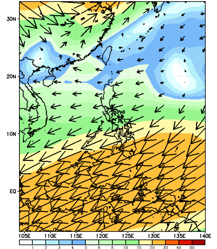
GEFS Week-1 200-hPa Wind Total Valid: 20230830 - 20230905
