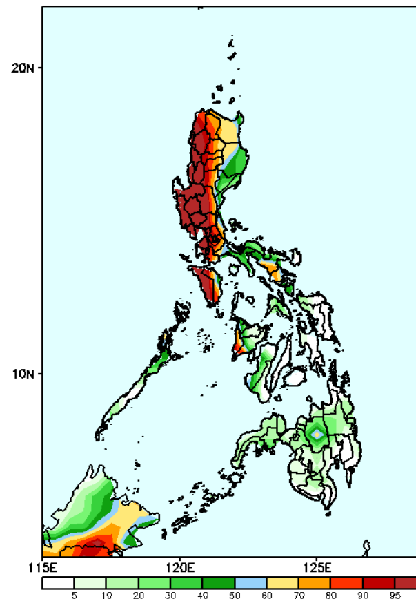
GEFS Week-1 Exceedance Prob. > 50mm Valid: 20230830 - 20230905
