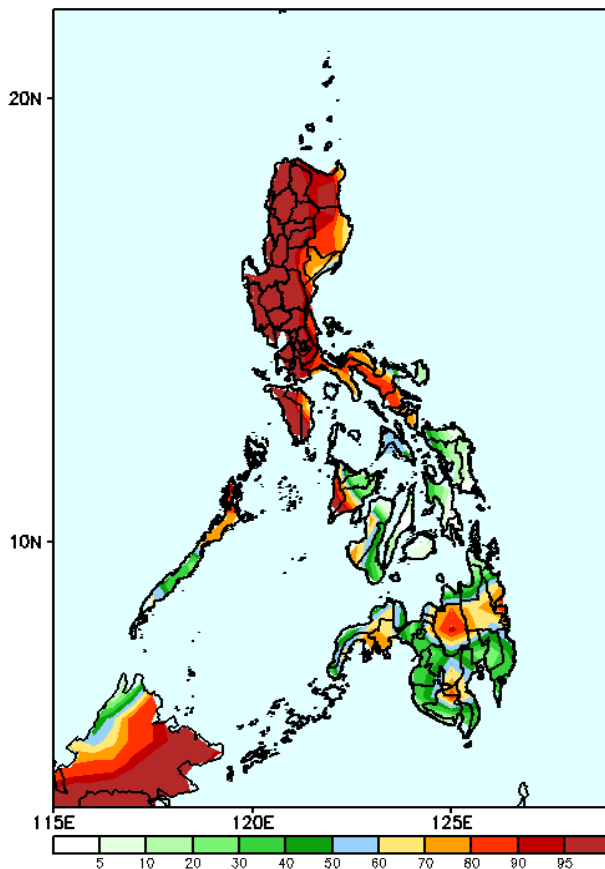
GEFS Week-1 Exceedance Prob. > 25mm Valid: 20230830 - 20230905
