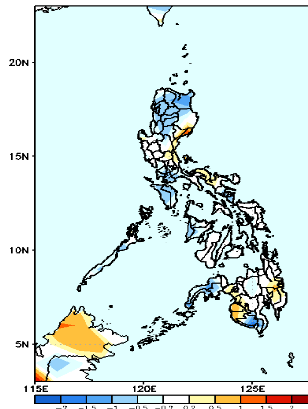
GEFS Week-2 T2m Anomaly Valid: 20230906 - 20230912
