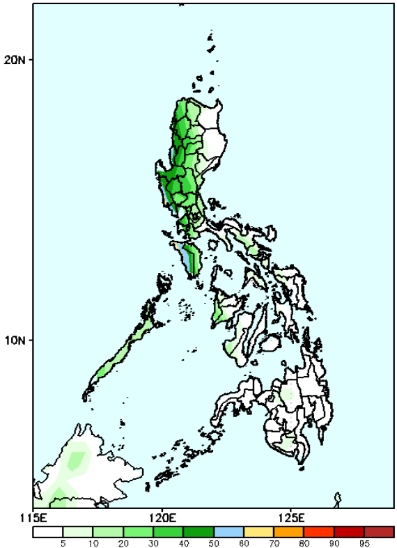
GEFS Week-2 Exceedance Prob. > 150mm Valid: 20230906 – 20230912
