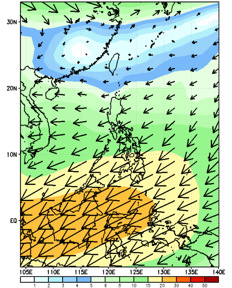
GEFS Week-2 200-hPa Wind Total Valid: 20230906 - 20230912
