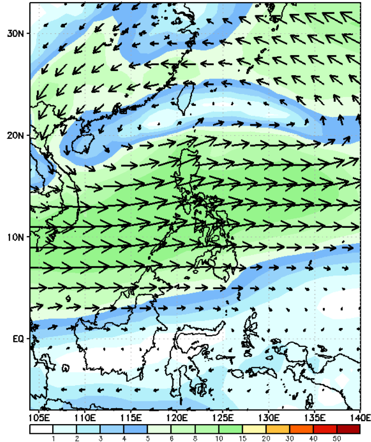
GEFS Week-1 700-hPa Wind Total Valid: 20230830 - 20230905
