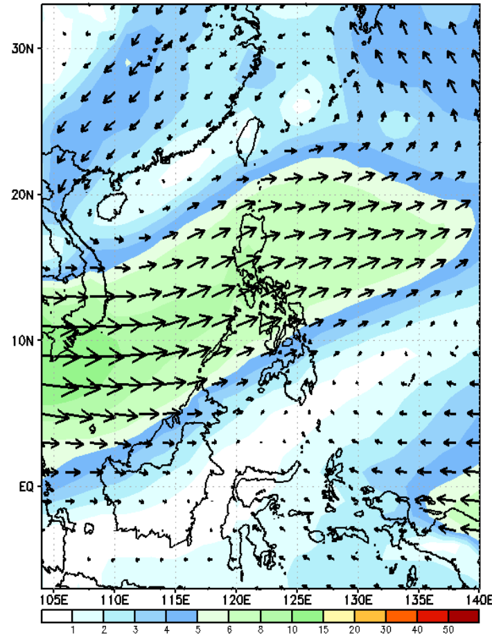
GEFS Week-2 700-hPa Wind Total Valid: 20230906 - 20230912
